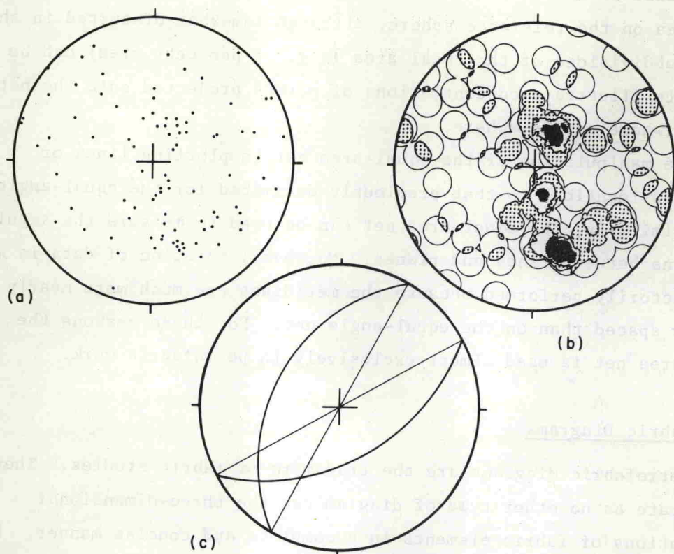
Fig. 6—Three types of petrofabric diagrams. (a) Point diagram illustrates the orientation of normals to 100 planar features or axes. (b) Contoured or density diagram of the points in (a); contours are at 1, 2, 4, and 6 per cent per 1 per cent area, 10 per cent maximum. (c) Stereogram shows two planes intersecting at 70 degrees. All diagrams are in lower hemisphere equal-area projection.
